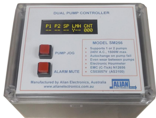
The SM256 in its IP66 enclosure
