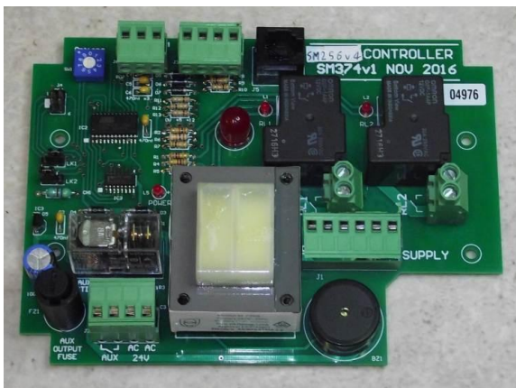
The SM256 Heavy Duty control module
